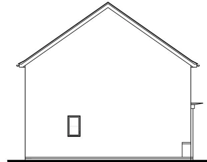
SIDE ELEVATION Windermere
