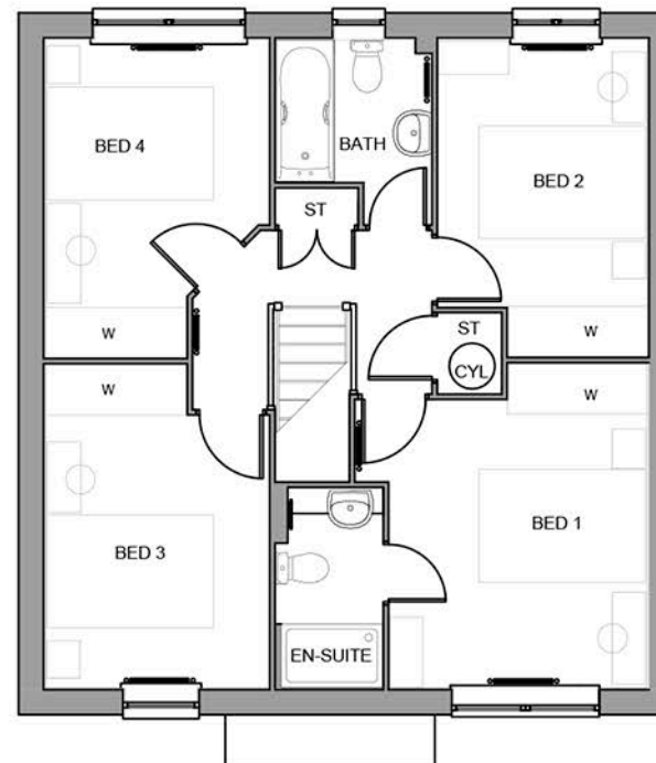
FIRST FLOOR PLAN Windermere
